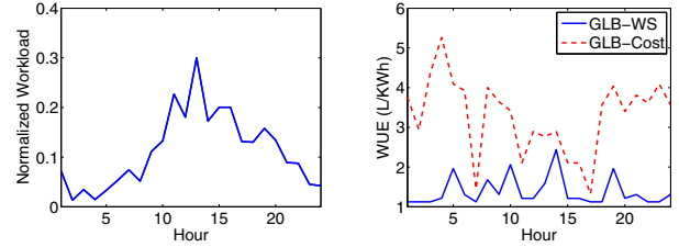
(a) FIU workload trace on May 1, 2012 (b) WUE comparison between GLB-WS and GLB-Cost
