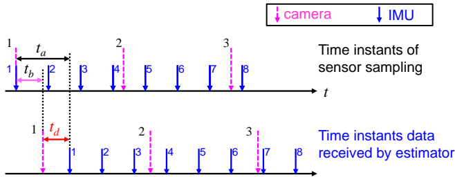
Fig. 1: Example of time offset arising due to latency in the sensor data. In this case the IMU data arrives with a latency t_a , while the camera data have a latency t_b , both of which are unknown. Since t_a and t_b are different, the estimator receives measurements that were recorded simultaneously (e.g., the first IMU and camera measurement) with timestamps that are offset by t_d = t_a - t_b .
