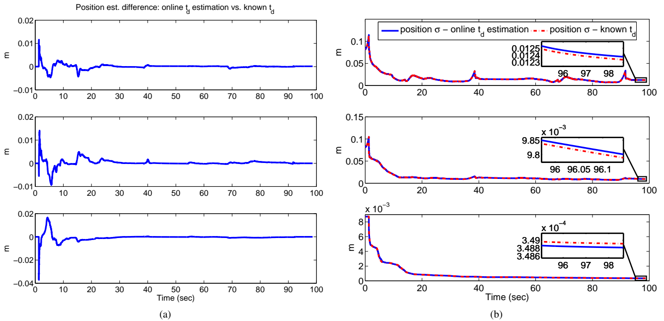
Fig. 5: Map-based localization: comparison of concurrent localization and t_d estimation vs. localization with known t_d . (a) The difference in the position estimates computed in the two cases. (b) The filter's reported standard deviation in the two cases.
