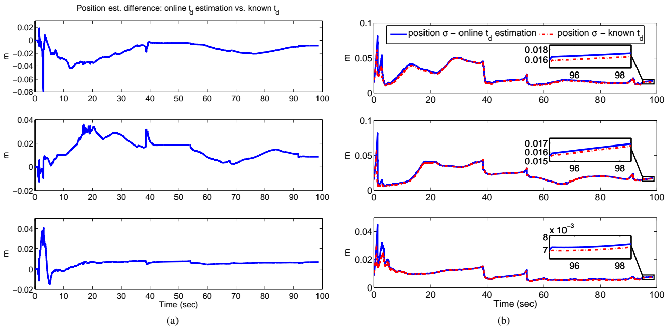
Fig. 7: EKF-SLAM localization: comparison of concurrent localization and t_d estimation vs. localization with known t_d . (a) The difference in the position estimates computed in the two cases. (b) The filter's reported standard deviation in the two cases.
