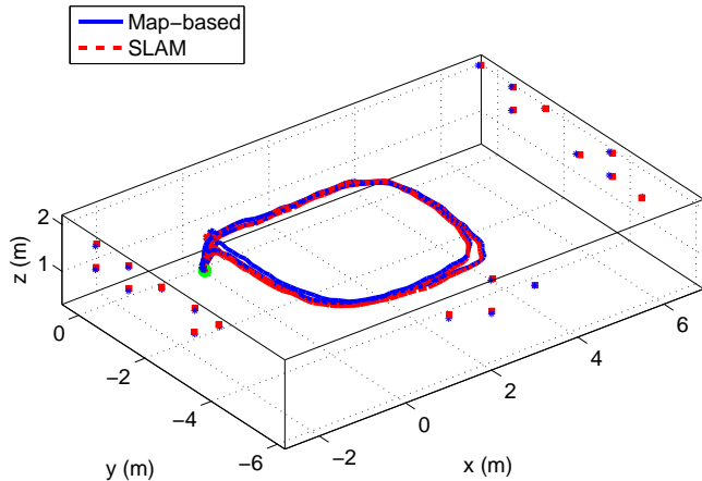
Fig. 3: Indoor experiment: trajectory estimates and feature positions. The blue line is the map-based trajectory estimate and the blue asterisks represent the known LED feature positions. The red dashed line is the SLAM trajectory estimate, and the red dots the SLAM estimates for the position of the LEDs.
