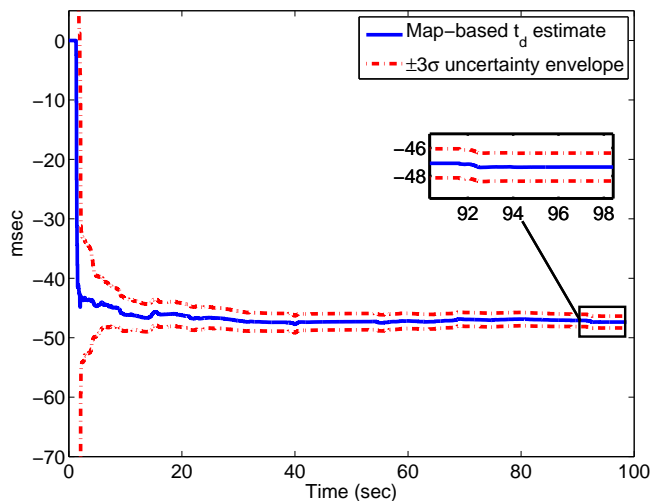
Fig. 4: Map-based experiment: time-offset estimate and corresponding \pm 3\sigma uncertainty envelope computed from the covariance matrix reported by the estimator.
