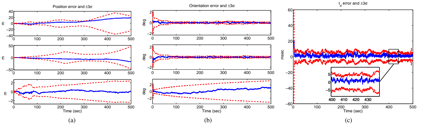
Fig. 10: Visual-inertial odometry with unknown features and drifting time-offset t_d : estimation errors (blue lines) and associated \pm 3\sigma envelopes (red dash-dotted lines). (a) The IMU position errors in the North, East, Down directions, (b) The IMU orientation errors in roll, pitch, and yaw, (c) The error in the estimate of t_d . Note that the position and yaw uncertainty gradually increases, as normal in visual-inertial odometry without any known landmarks.
