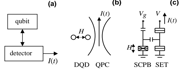
FIG. 1. (a) General schematic of a continuously measured solid-state qubit and two particular realizations of the setup: (b) a qubit made of double quantum dot (DQD) measured by a quantum point contact (QPC) and (c) a qubit based on single-Cooper-pair box (SCPB) measured by a single-electron transistor (SET).
