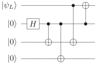
FIG. 3. Encoding circuit, which produces the state |z+\rangle from the state |\psi\rangle_L|0\rangle|0\rangle|0\rangle . Decoding can be done by running the same circuit backwards after step-1 measurement with the outcome “++.”
