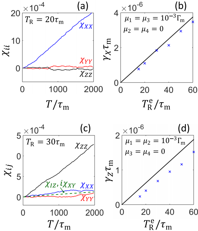
FIG. 7. The \chi -matrix elements and logical error rate for the case of qubit energy relaxation (amplitude damping). In panels (a) and (b) the energy relaxation affects only qubits 1 and 3, \mu_1 = \mu_3 = 10^{-3}\Gamma_m ; in panels (c) and (d) it affects only qubits 1 and 2, \mu_1 = \mu_2 = 10^{-3}\Gamma_m . Panels (a) and (c) show numerically calculated components of the \chi matrix as functions of time T ; the diagonal elements are depicted by solid lines. The only nonzero off-diagonal elements are \chi_{IZ} (real) and \chi_{XY} (imaginary) in panel (c), shown by (almost coinciding) dashed green lines. Panels (b) and (d) show, respectively, the logical error rates \gamma_X and \gamma_Z as functions of the response time T_R^e . The crosses represent numerical results and the solid lines represent analytical formulas (74) and (76). We used \Theta = 1 , \eta = 1 , \tau_c = \tau_{c,\text{opt}} , and the exponential kernel for the correlators.
