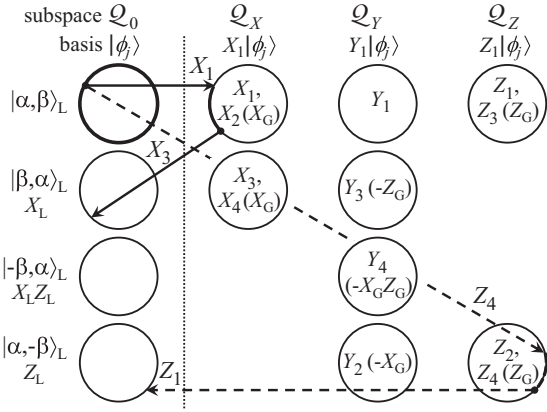
FIG. 4. State evolution and errors with continuous measurement. Thick-line circle illustrates diffusive evolution of the legitimate state [Eq. (39)] within two-dimensional subspace of the gauge qubit due to measurement. The 12 single-qubit errors move the legitimate state to eight other two-dimensional subspaces in Q_X , Q_Y , and Q_Z with the mapping described by Eq. (65) (see operators written inside the circles, the corresponding gauge qubit operations are in parentheses). If the second error occurs before the first error is detected (i.e., within the response time T_R ), it may move the state back to Q_0 , so that both errors remain undetected (dotted line separates Q_0 from error subspaces). Depending on a combination of the two errors, the logical qubit |\alpha, \beta\rangle_L may be affected by logical errors X_L , Y_L , or Z_L . The solid-line arrows illustrate a scenario of errors X_1 and X_3 , leading to logical error X_L ; the dashed-line arrows correspond to errors Z_4 and Z_1 , leading to Z_L .
