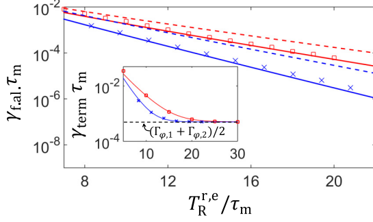
FIG. 5. The false alarm rate \gamma_{fal} as a function of the response time T_R^{r,e} (normalization involves the collapse time \tau_m ). Numerical results for the rectangular and exponential correlator integrations are shown by red squares and blue crosses, respectively. The (upper) red and (lower) blue dashed lines represent the analytics [Eqs. (99) and (98)]. The solid lines include correction factors in the analytical formulas (see main text). The inset shows the termination rate \gamma_{term} as a function of T_R^{r,e} (the same horizontal axis as in the main panel) for the case when qubits 1 and 2 are subject to pure dephasing with \Gamma_{\varphi,1} = \Gamma_{\varphi,2} = 10^{-3}\Gamma_m (no decoherence in the main panel); the horizontal dashed line corresponds to single-qubit errors \gamma_{term} = (\Gamma_{\varphi,1} + \Gamma_{\varphi,2})/2 . We used \Theta = 1 , \eta = 1 , and \tau_c = \tau_{c,opt} .
