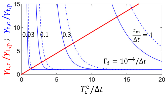
FIG. 8. Tradeoff between the logical error rate and termination rate for the Bacon-Shor code with continuous measurements. Thick red line: ratio \gamma_{L,\text{cont}}/\gamma_{L,\text{proj}} of the logical error rates for continuous and projective measurements [Eq. (113)], as a function of the correlator integration time T_c^e normalized by the projective-measurement half-cycle time \Delta t . Thin blue lines: ratio \gamma_{\text{term,cont}}/\gamma_{\text{term,proj}} of the termination rates for the continuous and projective measurements [Eq. (114)] for several values of the collapse (“measurement”) time \tau_m : \tau_m/\Delta t = 1, 0.3, 0.1 , and 0.03 (from right to left) and quantum efficiency \eta = 1 (solid lines) or \eta = 0.5 (dashed lines). We assume \Gamma_d = 10^{-4}/\Delta t and \Theta = 1 .
