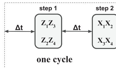
FIG. 2. One cycle of the code operation with projective measurement of gauge operators: at step 1 the operators Z_1Z_3 and Z_2Z_4 are measured instantaneously, and at step 2 the operators X_1X_2 and X_3X_4 are measured (also instantaneously). The duration of each time step is \Delta t , so the cycle duration is 2\Delta t . In the absence of errors, product of two measurement results ( \pm 1 ) at each step is +1 .
