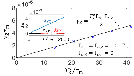
FIG. 6. The rate \gamma_Z of the logical Z error as a function of the response time T_R^e for the case when qubits 1 and 2 are subject to pure dephasing with \Gamma_{\varphi,1} = \Gamma_{\varphi,2} = 10^{-3}\Gamma_m . The crosses show numerical results, the solid line is the analytical result (72). The inset shows the diagonal elements of the process matrix ( \chi_{XX} , \chi_{YY} , and \chi_{ZZ} ) as functions of time T for T_R^e = 20.8\tau_m . The rate \gamma_Z is calculated from the slope of \chi_{ZZ}(T) . We used \Theta = 1 , \eta = 1 , \tau_c = \tau_{c,opt} , and the exponential kernel for the correlators.
