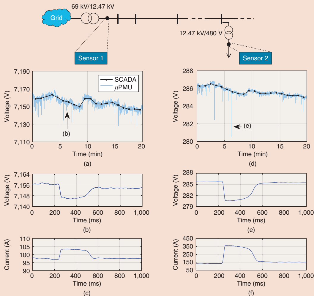
figure 1. An example of \mu PMU readings compared to a standard SCADA or meter reading: (a) SCADA and \mu PMU measurements at sensor location 1, (b) the voltage magnitude measurement by \mu PMU at sensor location 1 after zooming in, (c) the current magnitude measurement by \mu PMU at sensor location 1 after zooming in, (d) SCADA and \mu PMU measurements at sensor location 2, (e) the voltage magnitude measurement by \mu PMU at sensor location 2 after zooming in, and (f) the current magnitude measurement by \mu PMU at sensor location 2 after zooming in.
