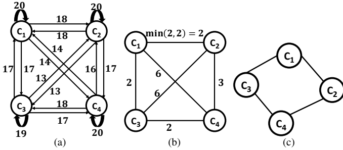
Figure 3: a) Example of adjacency graph of a quad-core CPU. b) Reduced uni-directed graph c) Final CPU affinity graph.
